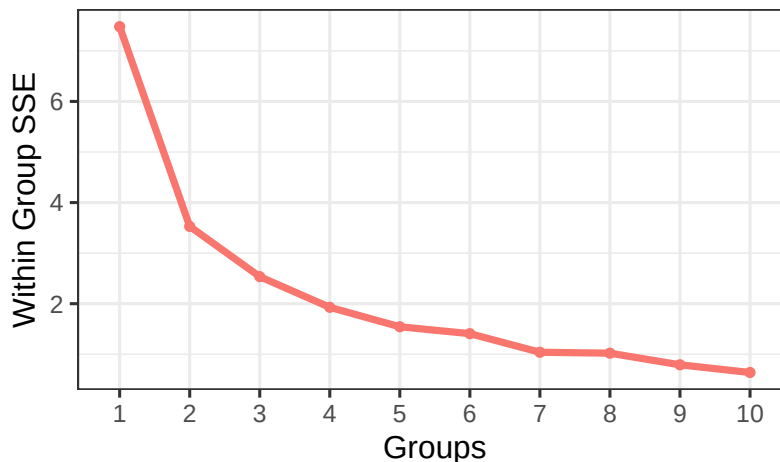
Figure C-2: Relationship between number of groups and within-group sum of squared errors
