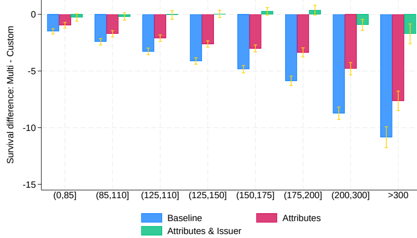
Figure 5: Adverse selection and security customization by loan size bins
