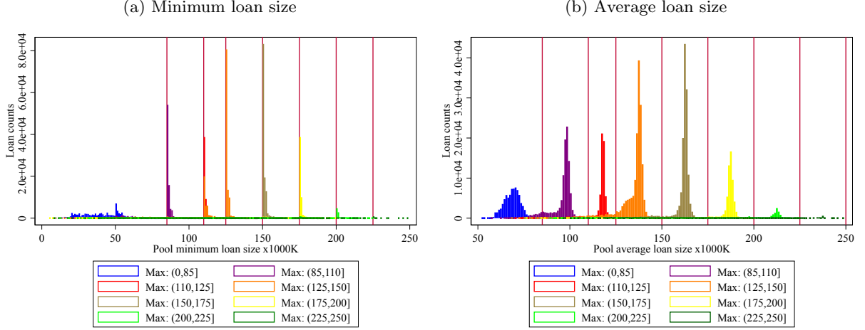
Figure 2: Distribution of loan size across spec-pools
