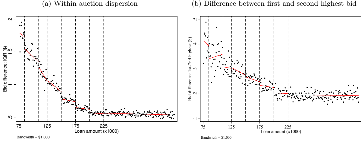
Figure 8: Within auction dispersion in bids across loan-size bins
