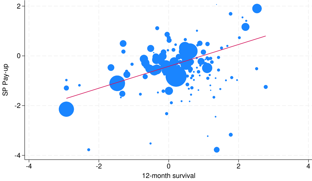
Figure 6: Relationship between average spec-pool pay-up and short-run survival across issuers
