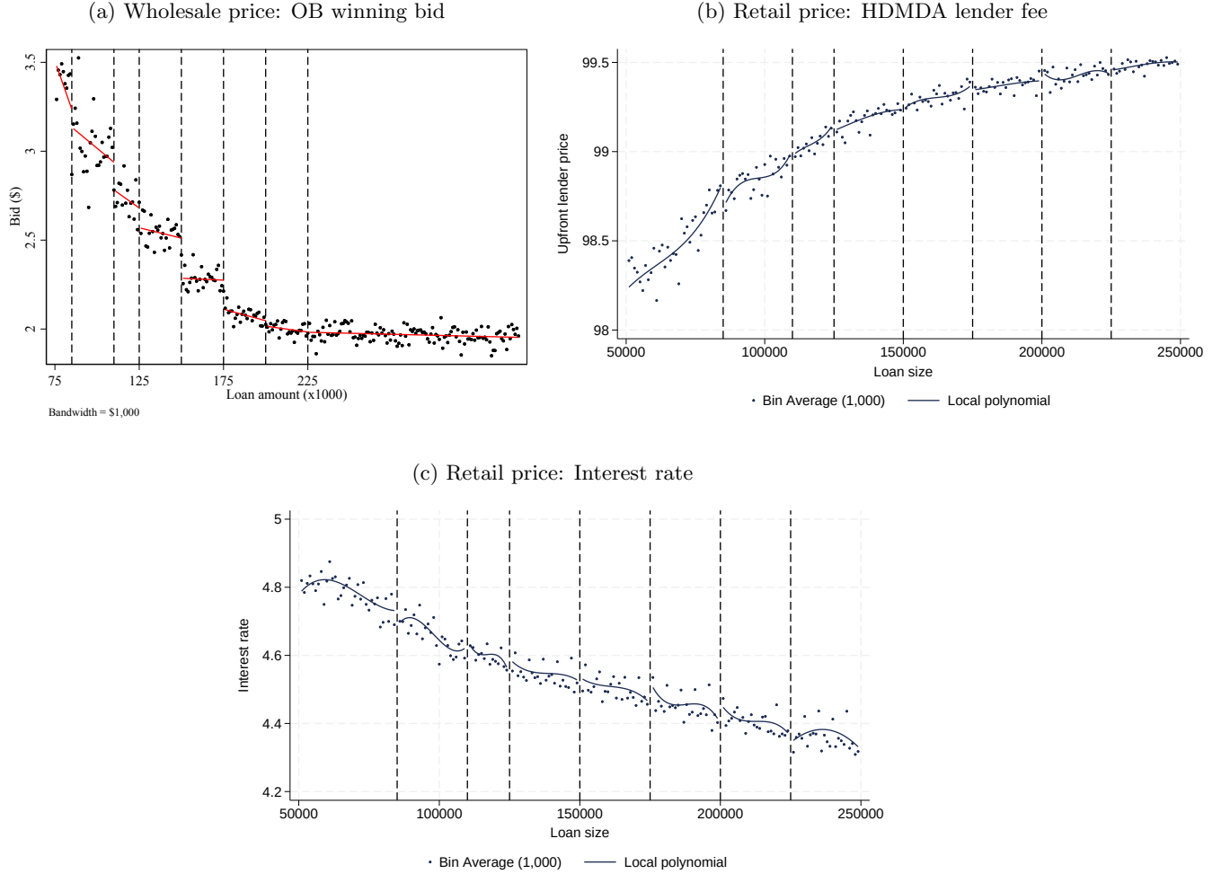
Figure 7: Evidence of discontinuity in wholesale and retail loan prices
