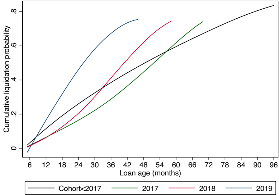
Figure 9: Evolution of pre-payment risk across cohorts
