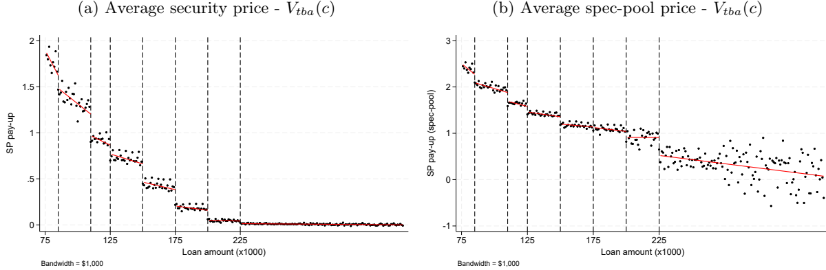
Figure 3: Evidence of discontinuities in security prices
