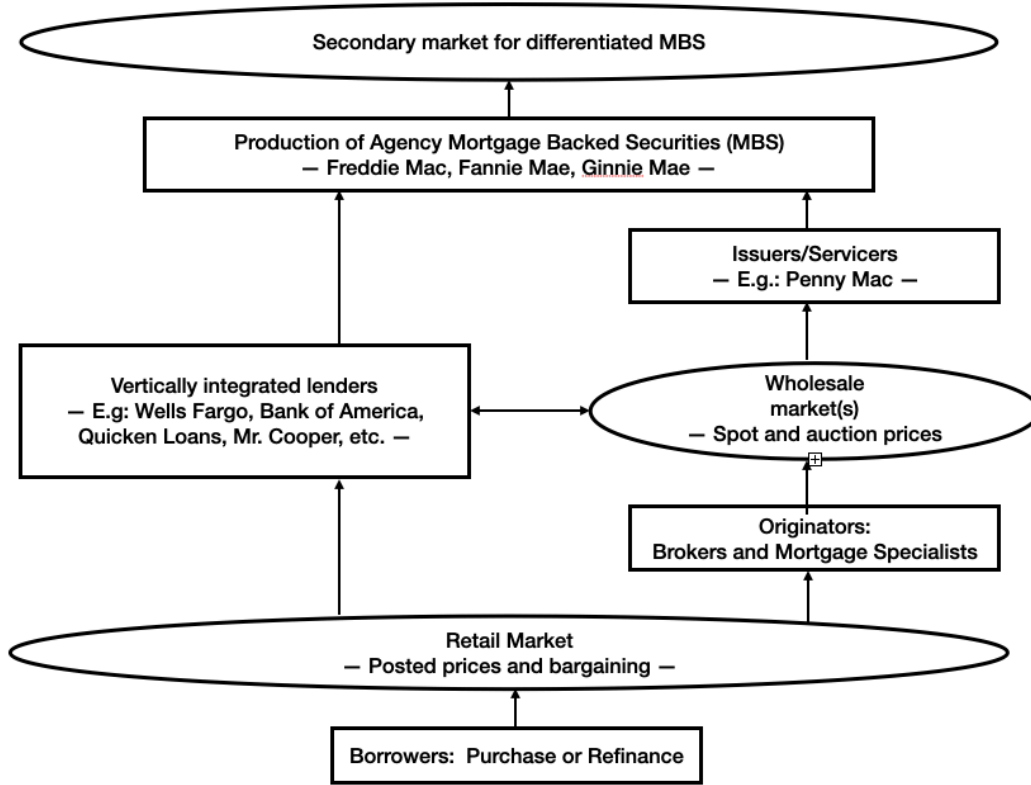
Figure 1: Supply chain of mortgages in U.S.
